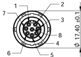
8-PIN Male Circular Connector (as accessory)
